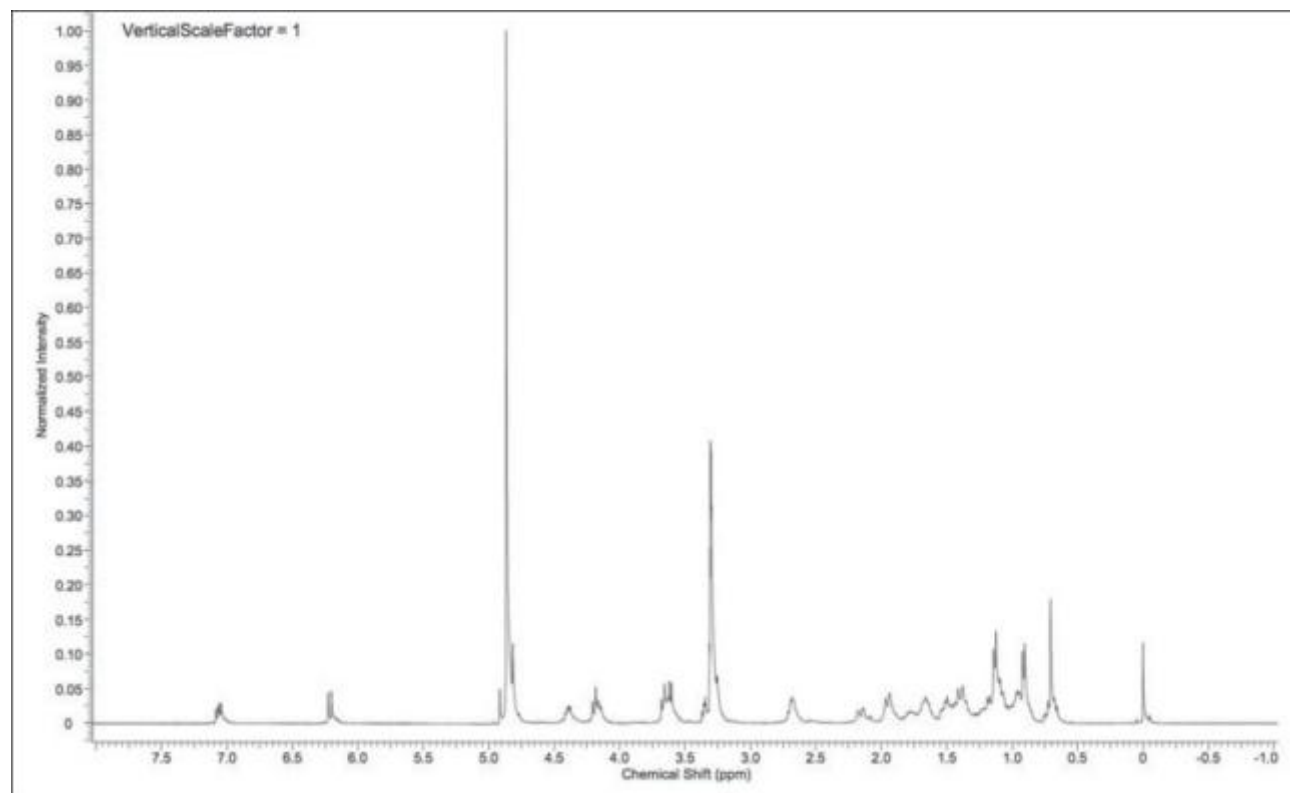
Figure-2. ^1\text{H} NMR spectra of physagulin V. The spectrum was obtained at 400 MHz in MeOD at 27 °C with an acquisition time of 3.9715 s.
