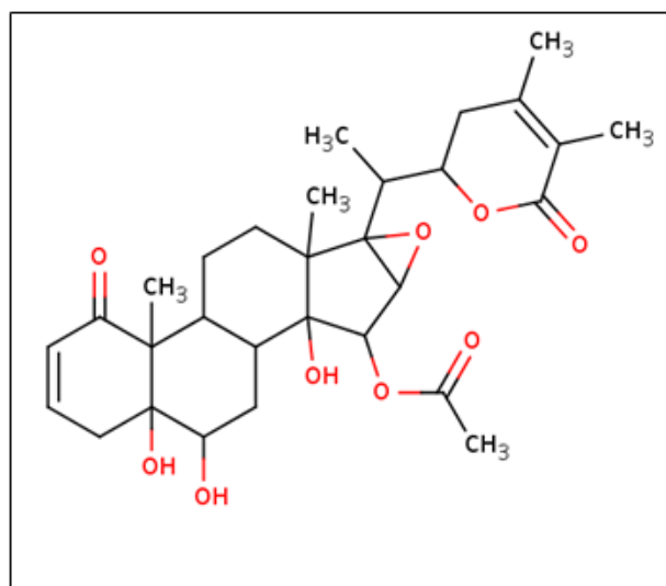
Figure-3. Molecular structure Physagulin-F isolated form Physalis angulate
