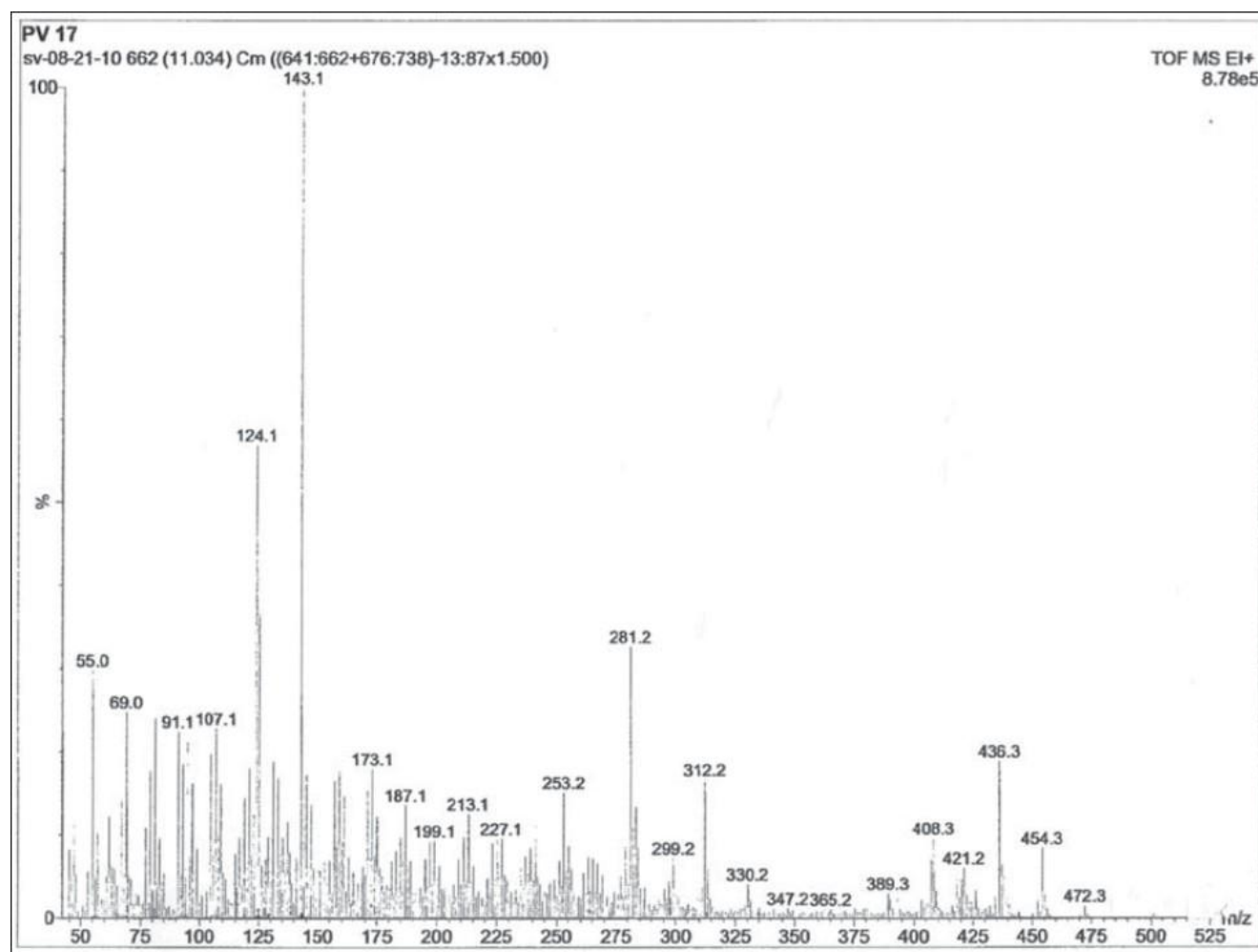
Figure-1. MS of Physagulin-F
